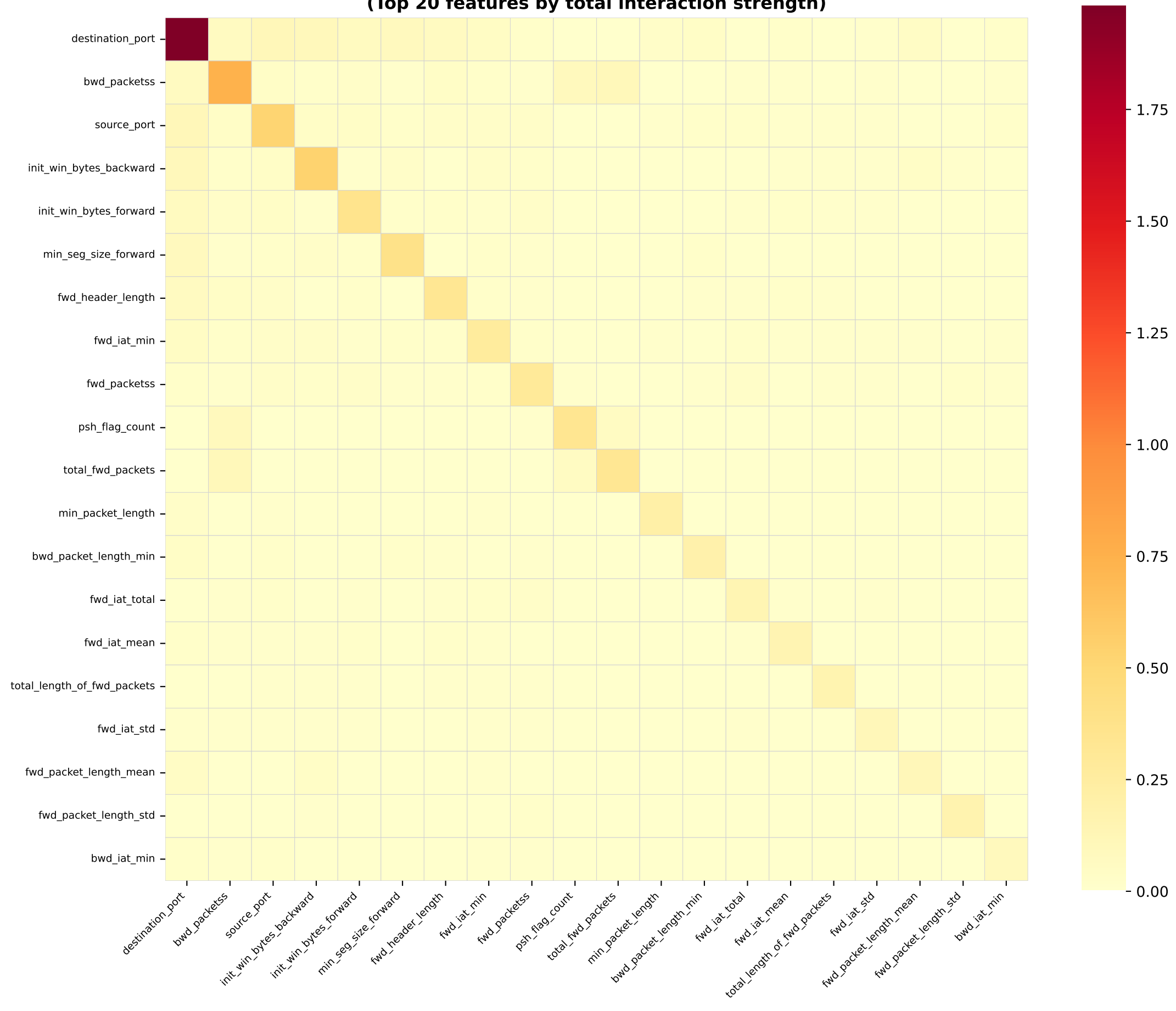
SHAP Interaction Values — XGB on IDS2025_Balanced (Top 20 features by total interaction strength)
